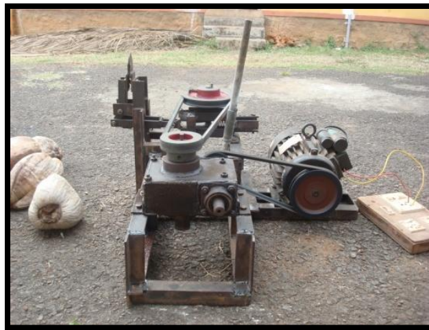
Plate 2.5 Power operated coconut husking machine
