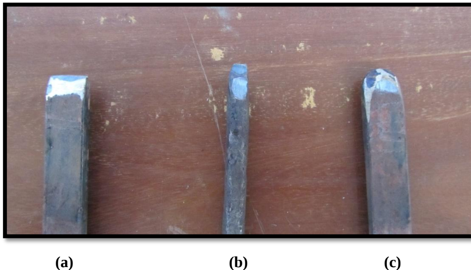
Plate 3.4 Different shape of blades used for testing (a. bevel edged b. pointed edged c. round edged)
