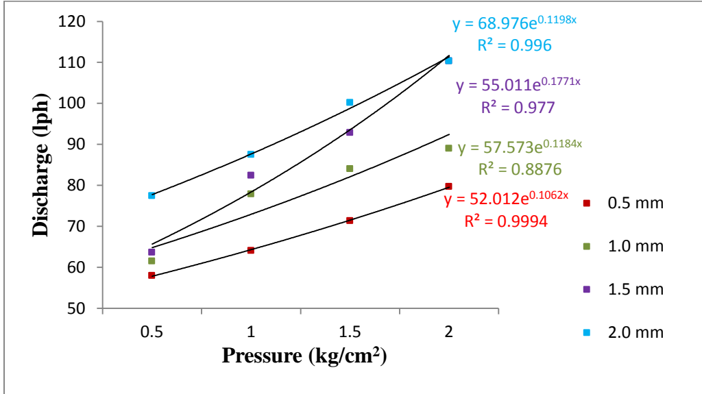
Fig. 4.48 Mean discharge of SMMS at various operating pressures
