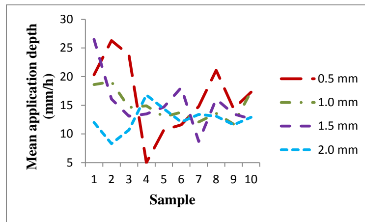
Fig. 4.45 Mean application depth of FMMS at 1.0 kg/cm 2
