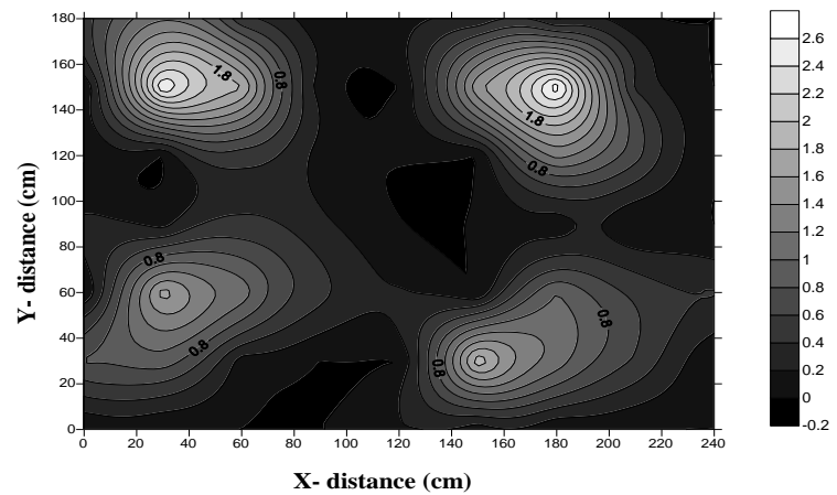
Fig. 4.19 Water distribution pattern of 0.5 mm wide cut FDMS at 2.0 \text{ kg/cm}^2
