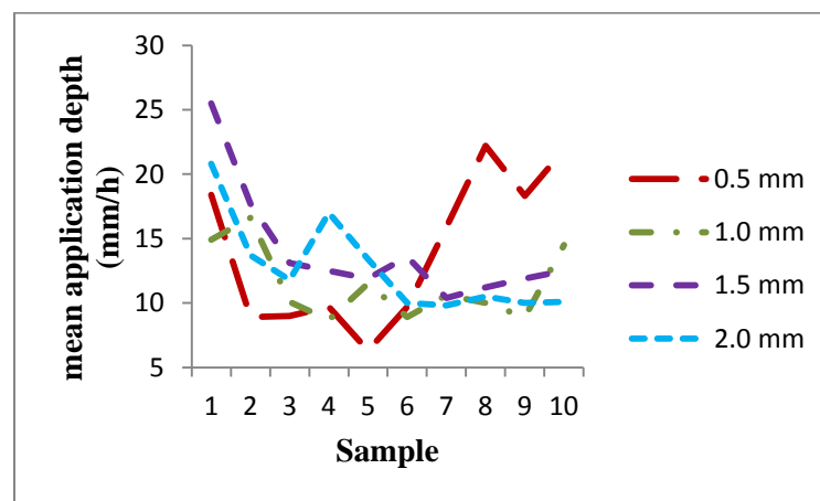
Fig. 4.47 Mean application depth of FMMS at 2.0 kg/cm 2
