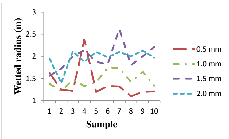
Fig. 4.39 Wetted radius of FMMS at 0.5 kg/cm 2
