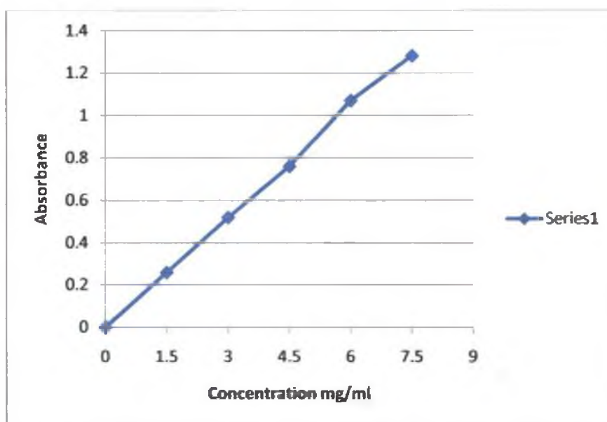
Fig. 4.20 Standard curve for cyanide estimation
