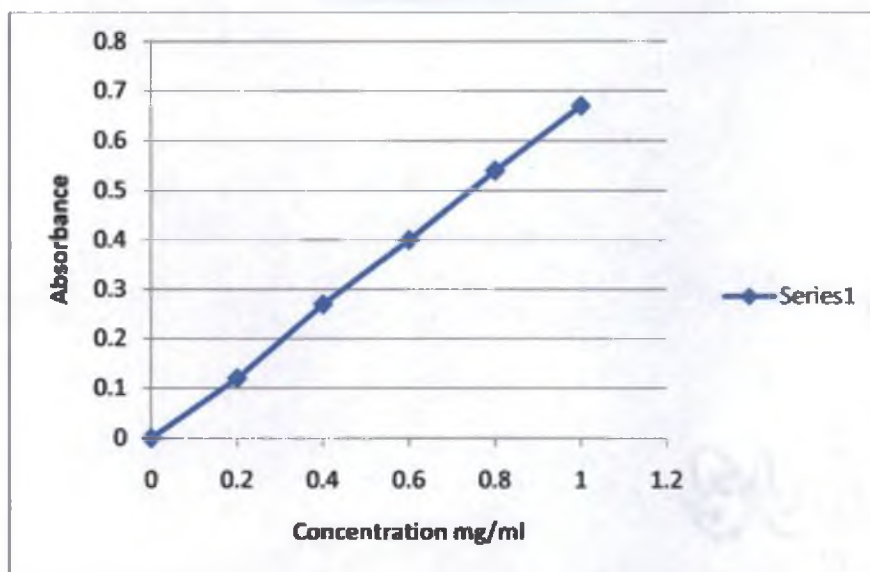
Fig. 4.14 Standard curve for carbohydrate estimation
