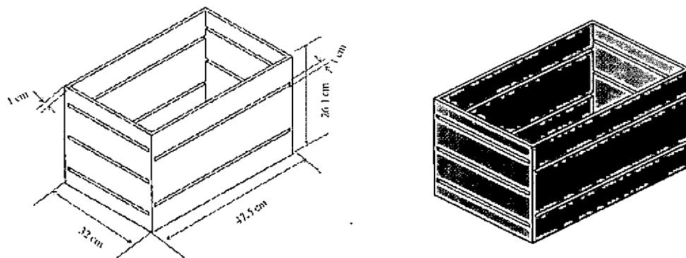
Fig. 4.1 Developed wooden box Plate 4.1 Wooden storage system for cassava
