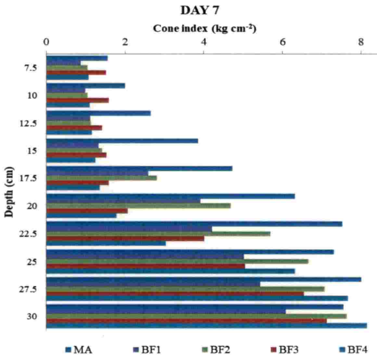
Fig. 4.25 Variation of cone index with depth in different bunds formed with NH 3230 on Day 7 at Tavanur
