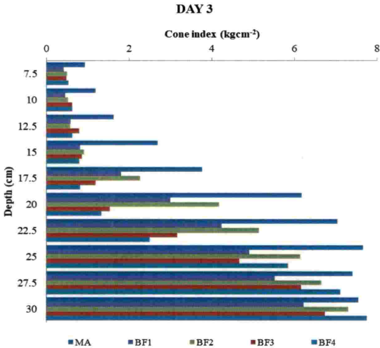
Fig. 4.24 Variation of cone index with depth in different bunds formed with NH 3230 on Day 3 at Tavanur
