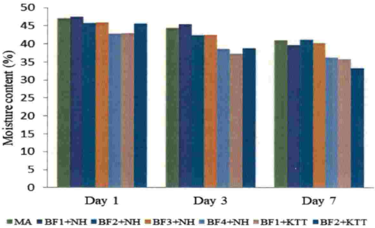
Fig. 4.35 Changes in moisture content of the different bundles at Tavanur
