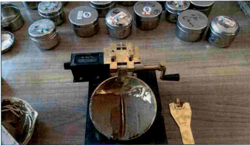
Plate 3.5 Determination of liquid limit
