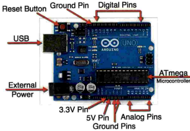
Fig 3.10 Arduino Uno board with pin configuration
