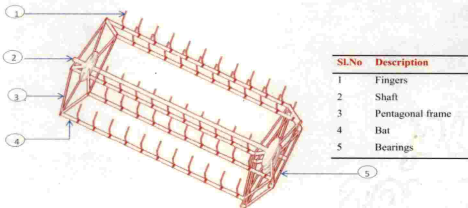
Isometric view
