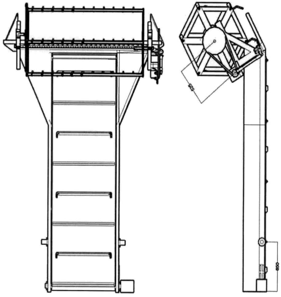
Fig. 9. Front conveyor with Reel and cutter bar assembly of the KAU Pokkali paddy harvester
