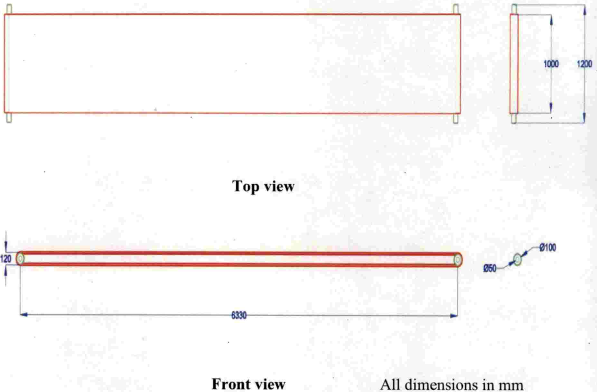
Fig. 3.12 Centre conveyor of the existing prototype
