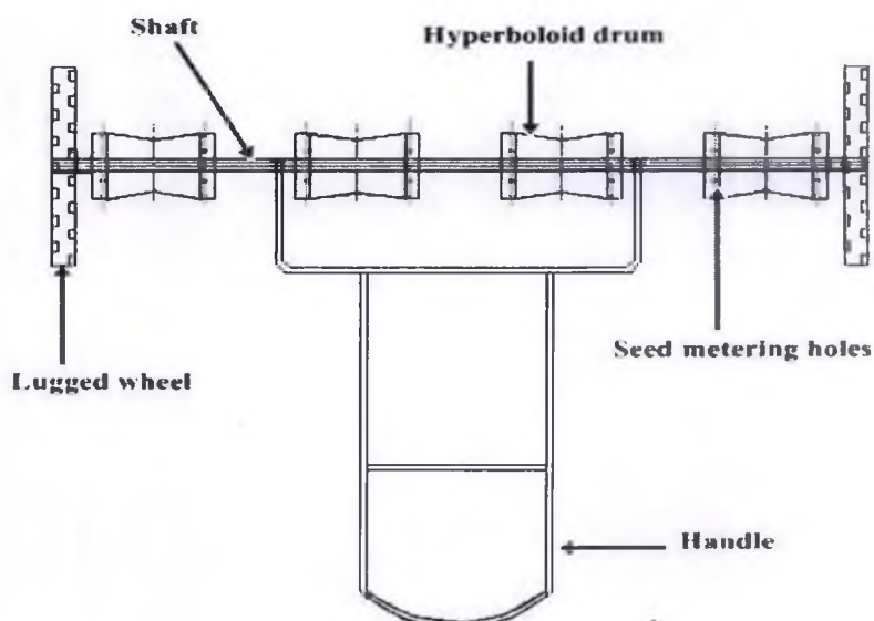
Fig 3.1 Schematic of Direct paddy seeder
