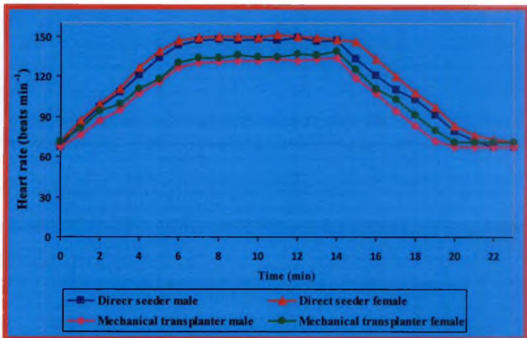
Fig 4.1 Mean heart rate and recovery pattern during the operation of selected equipments
