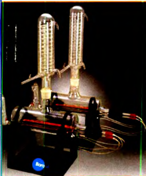
Water Distillation Purification Unit
