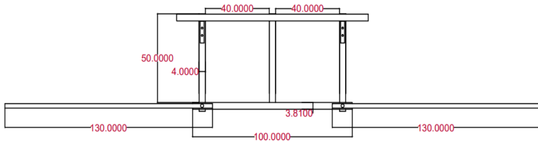
Fig. 4.16 Constructional details of the sprayer assembly
