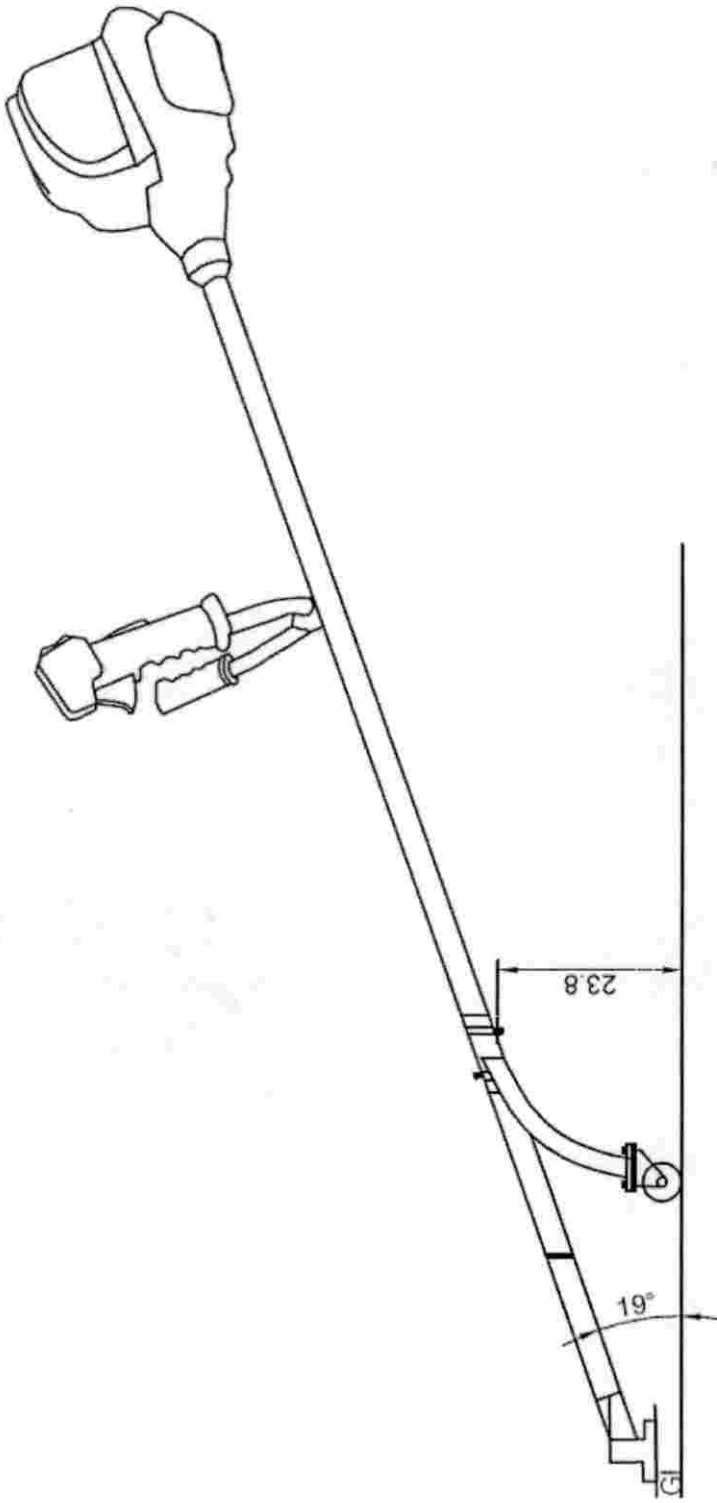
All dimensions are in cm Figure 3.7 Side view of developed vibration reducing aid attached to brush cutter shaft
