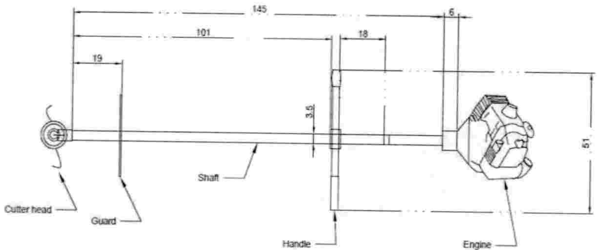
Figure 3.1 Plan of the selected brush cutter with dimensions
