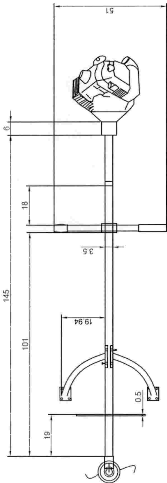
Figure 3.6 Plan of developed vibration reducing aid attached to the brush cutter shaft
