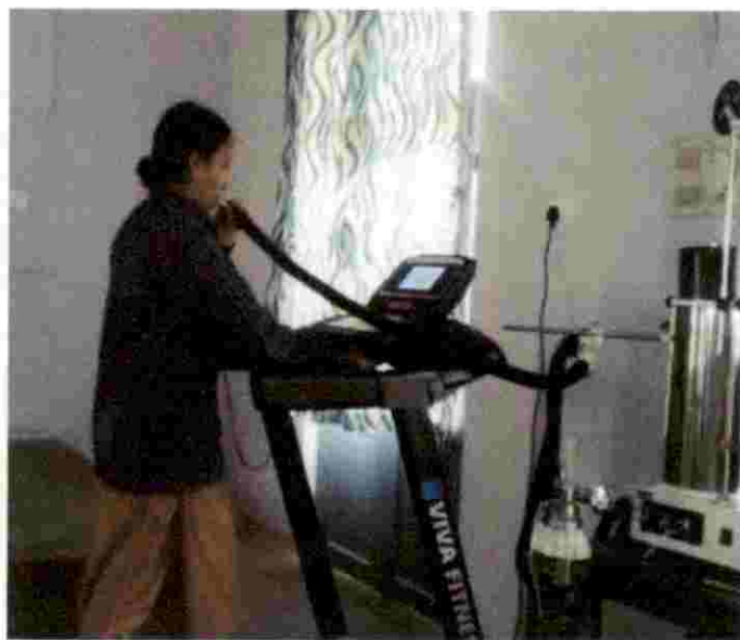
Plate 3.14 Calibration Process
