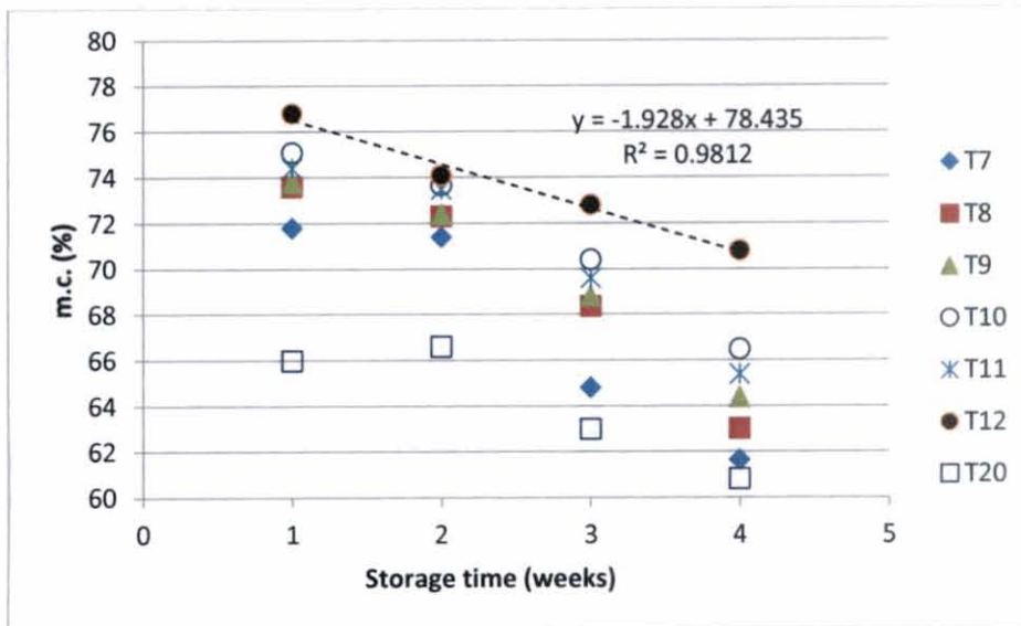
Fig. 4.15 Change in pulp m.c of uncoated fruits
