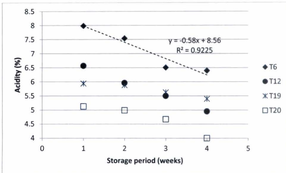
Fig. 4.9 Change in acidity of coated/uncoated samples
